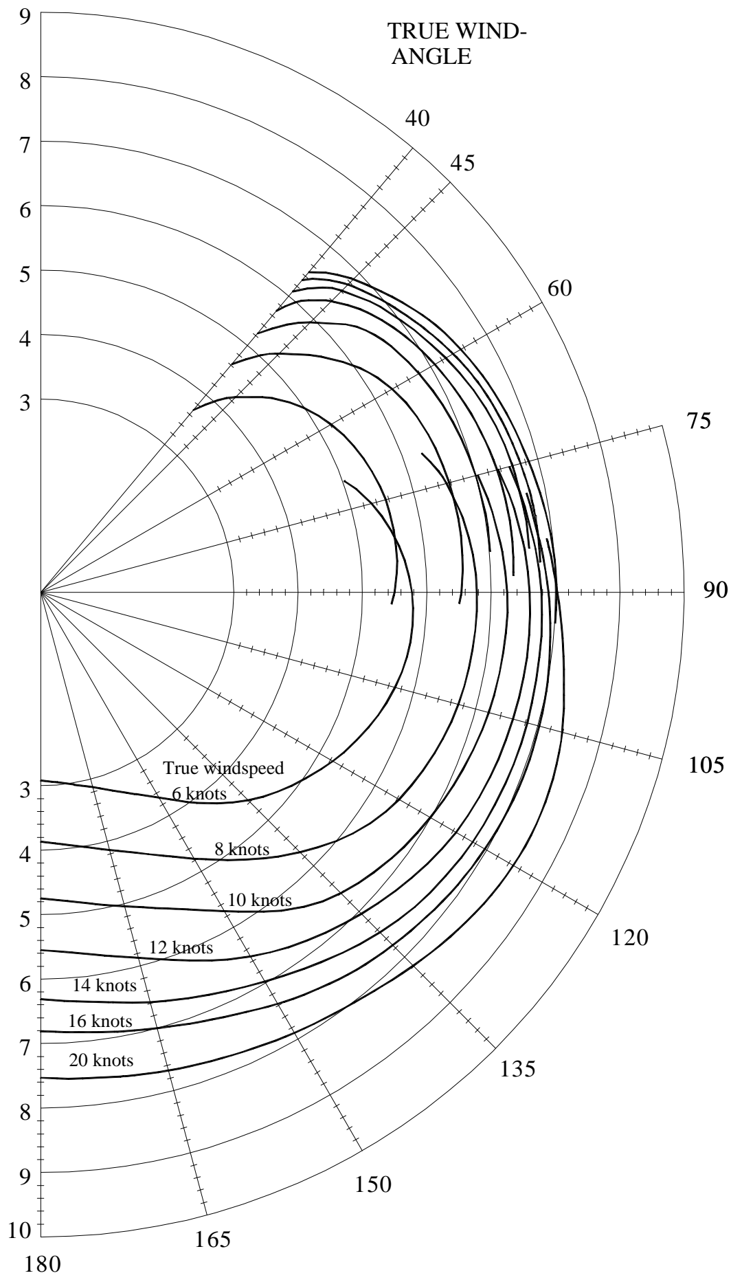
PREDICTED PERFORMANCE FOR REGINA 38
